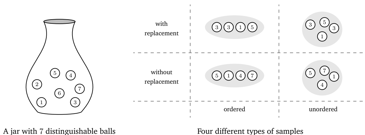
Figure 3.9: Drawing a sample of size 4 from a jar with 7 balls
