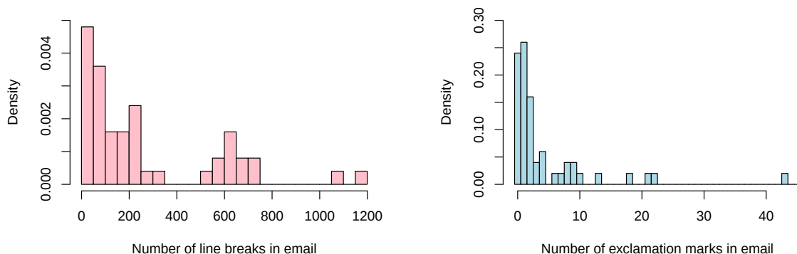
Figure 2.4: Histograms of variables line_breaks and exclam_mess from the emails data set
